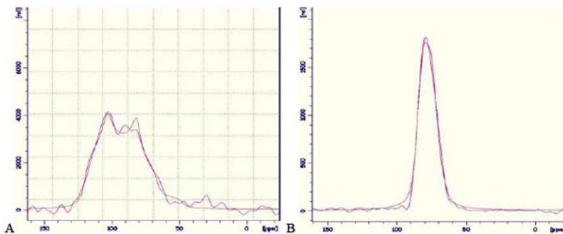
Figure 17.10: Slices and Simulations of the 18.8 T ^{17}\text{O} MQ-MAS of \text{NaPO}_3
