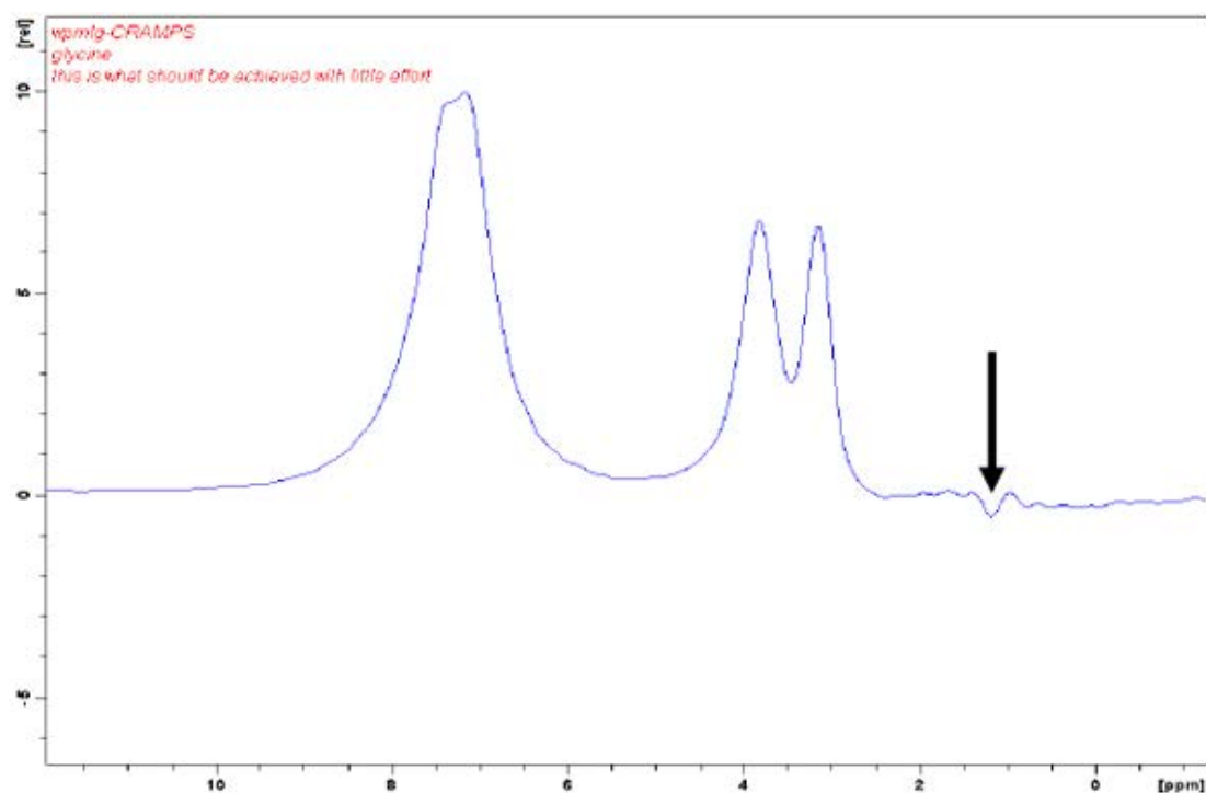
Figure 22.9: WPMLG-CRAMPS After Optimization, Digital Acquisition
