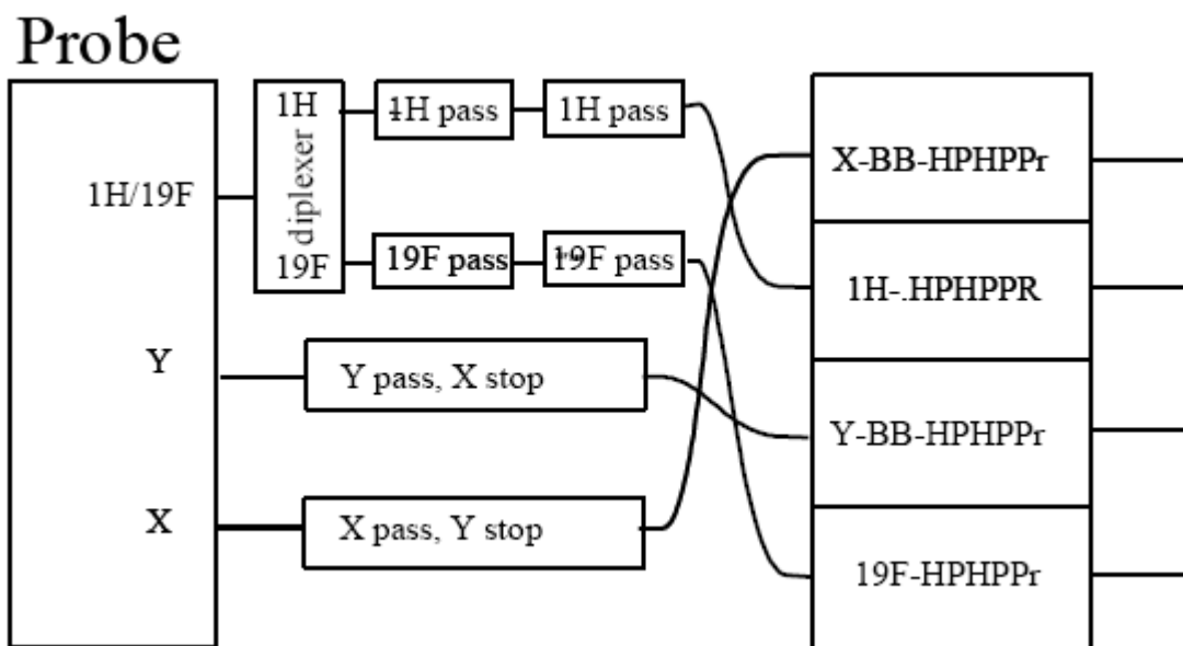
Figure 3.12: Quadruple Resonance HFX Y Experiment (WB probes \geq 400 MHz only!)
