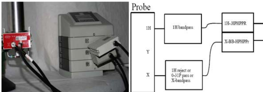
Figure 3.7: Standard CP Experiment, Proton Preamplifier in Line
