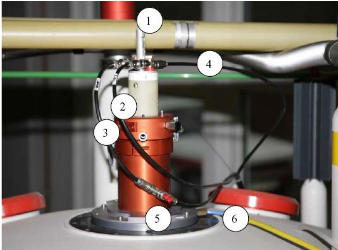
Figure 3.17: WB Probes: Eject/Insert Connections
