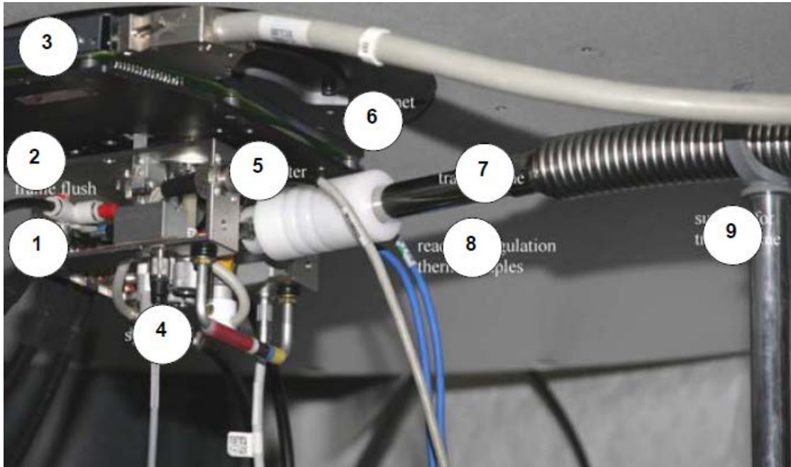
Figure 3.30: Bottom view of Low Temperature DVT Probe/Heat Exchanger
